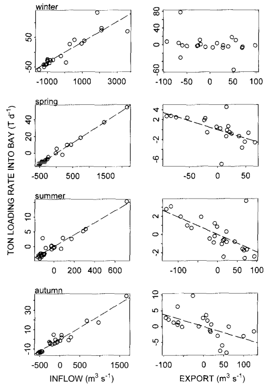
Figure 7. Partial residual plots of TON loading rate into Bay versus total river inflow and total water export, by season. Dotted line, linear regression fit ( p < 0.05 ).
